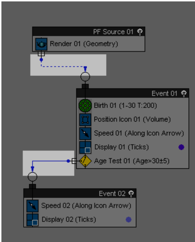
Wire from global event to birth event (above); wire from test to local event (below)
