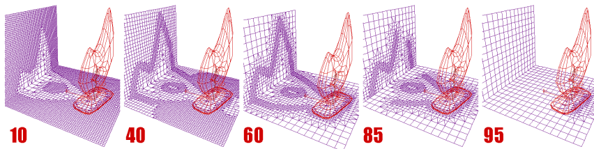
Radiosity solutions with different Contrast Threshold values. The best solution is at the center, with Contrast Threshold=60.
