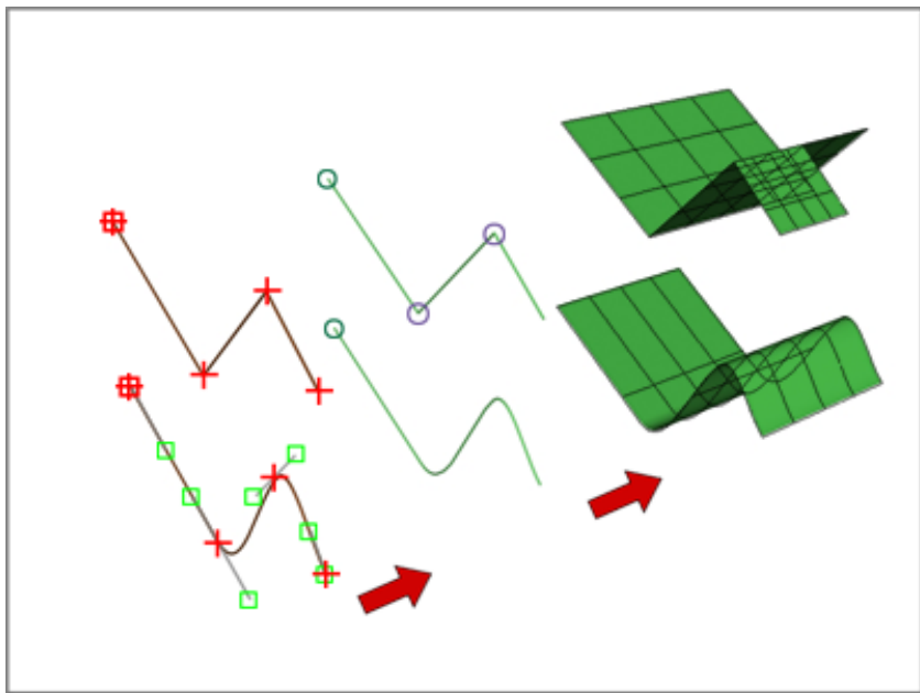
Splines become NURBS curves that then become NURBS surfaces.
