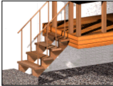
Left: The carriage springing from the floor. (Spring From Floor turned on.)
