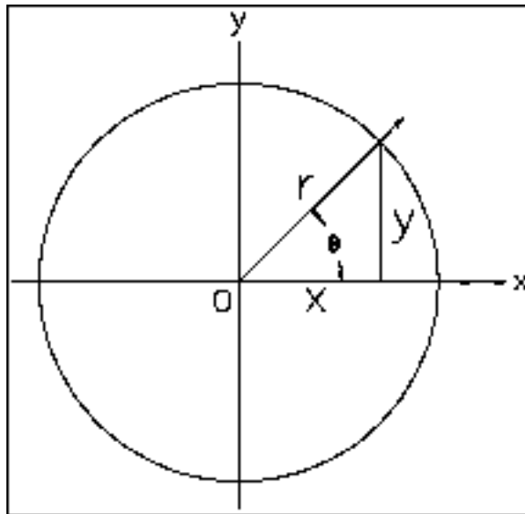
Trigonometric functions based on the unit circle
