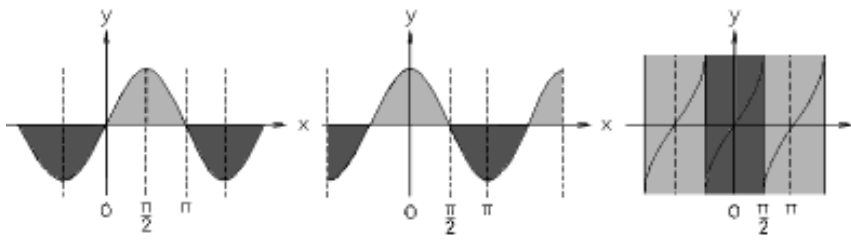
Graphs of basic trigonometric functions
