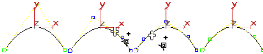
Refining a NURBS curve.
