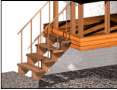
Left: The carriage springing from the floor. (Spring From Floor on.)
