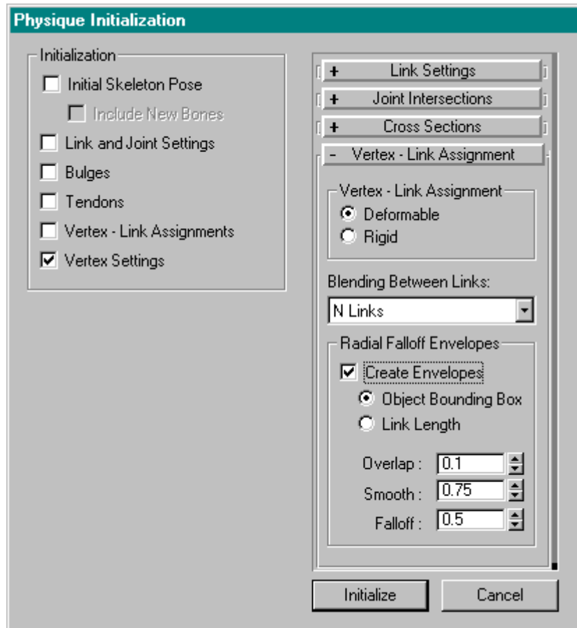
Reinitialization mode of Initialization dialog
