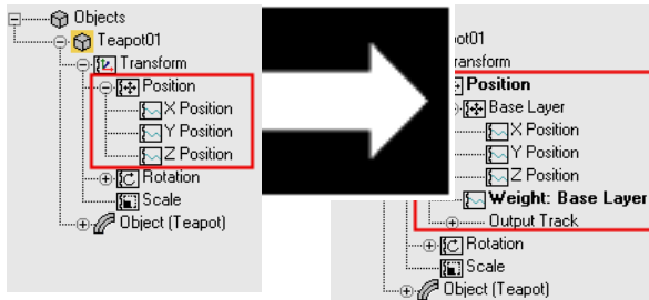
The original controller before you enable animation layers
