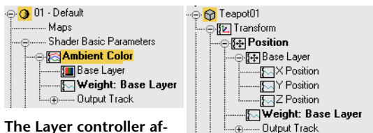
The Layer controller affects a leaf track.
