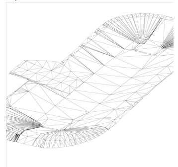
Pond plan for intersection of 180th Street SE and Snohomish Avenue
